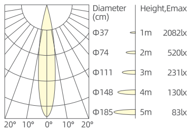
9W/15°/3000K/Ra90
