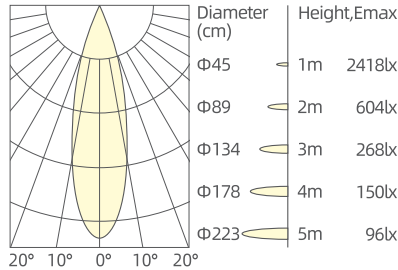
2x4W/24°/3000K/Ra90
