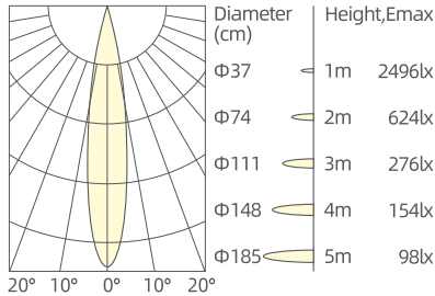
2x4W/15°/3000K/Ra90
