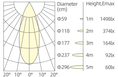
2x4W/36°/3000K/Ra90
