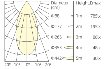
10W/55°/3000K/Ra90
