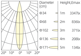
10W/15°/3000K/Ra90
