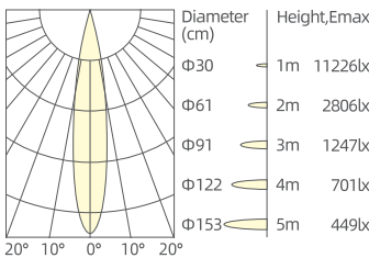
25W/15°/3000K/Ra90
