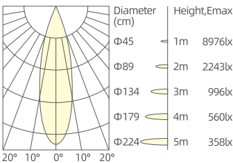
25W/24°/3000K/Ra90
