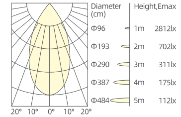
25W/50°/3000K/Ra90
