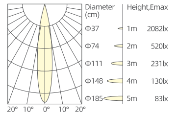
9W/15°/3000K/Ra90
