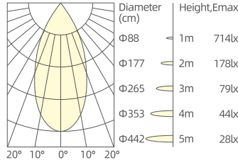
10.5W/50°/3000K/Ra90
