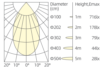
10W/55°/3000K/Ra90
