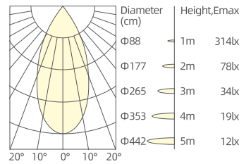
4W/50°/3000K/Ra90
