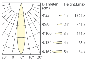
5W/15°/3000K/Ra90
