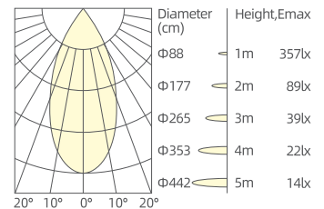
5W/50°/3000K/Ra90
