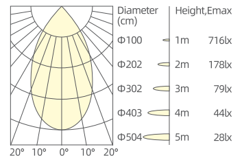
3x10W/55°/3000K/Ra90
