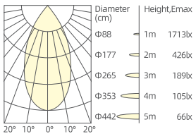
3x7W/45°/3000K/Ra90
