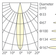
5x9W/15°/3000K/Ra90
