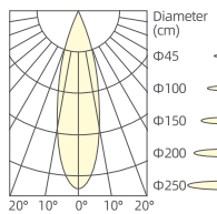
5x9W/24°/3000K/Ra90
