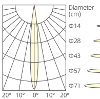
5x9W/10°/3000K/Ra90
