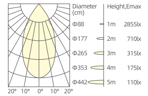
5x9W/45°/3000K/Ra90
