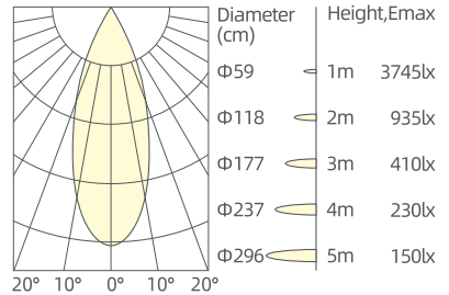
5x4W/36°/3000K/Ra90
