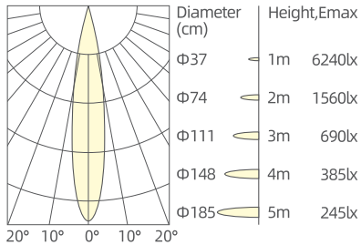
5x4W/15°/3000K/Ra90
