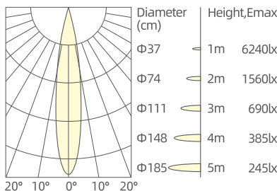
5x4W/15°/3000K/Ra90
