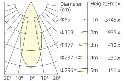
5x4W/36°/3000K/Ra90
