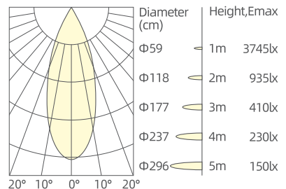
5x4W/36°/3000K/Ra90
