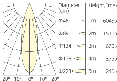
5x4W/24°/3000K/Ra90
