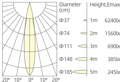
5x4W/15°/3000K/Ra90
