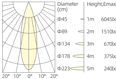
5x4W/24°/3000K/Ra90
