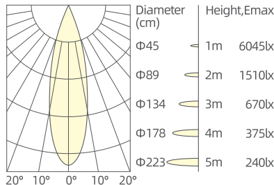
5x4W/24°/3000K/Ra90
